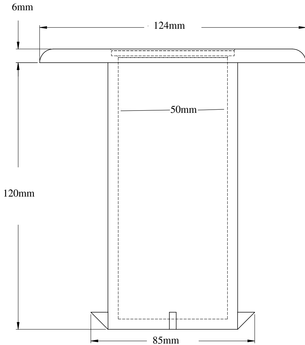
PROFILE VIEW
